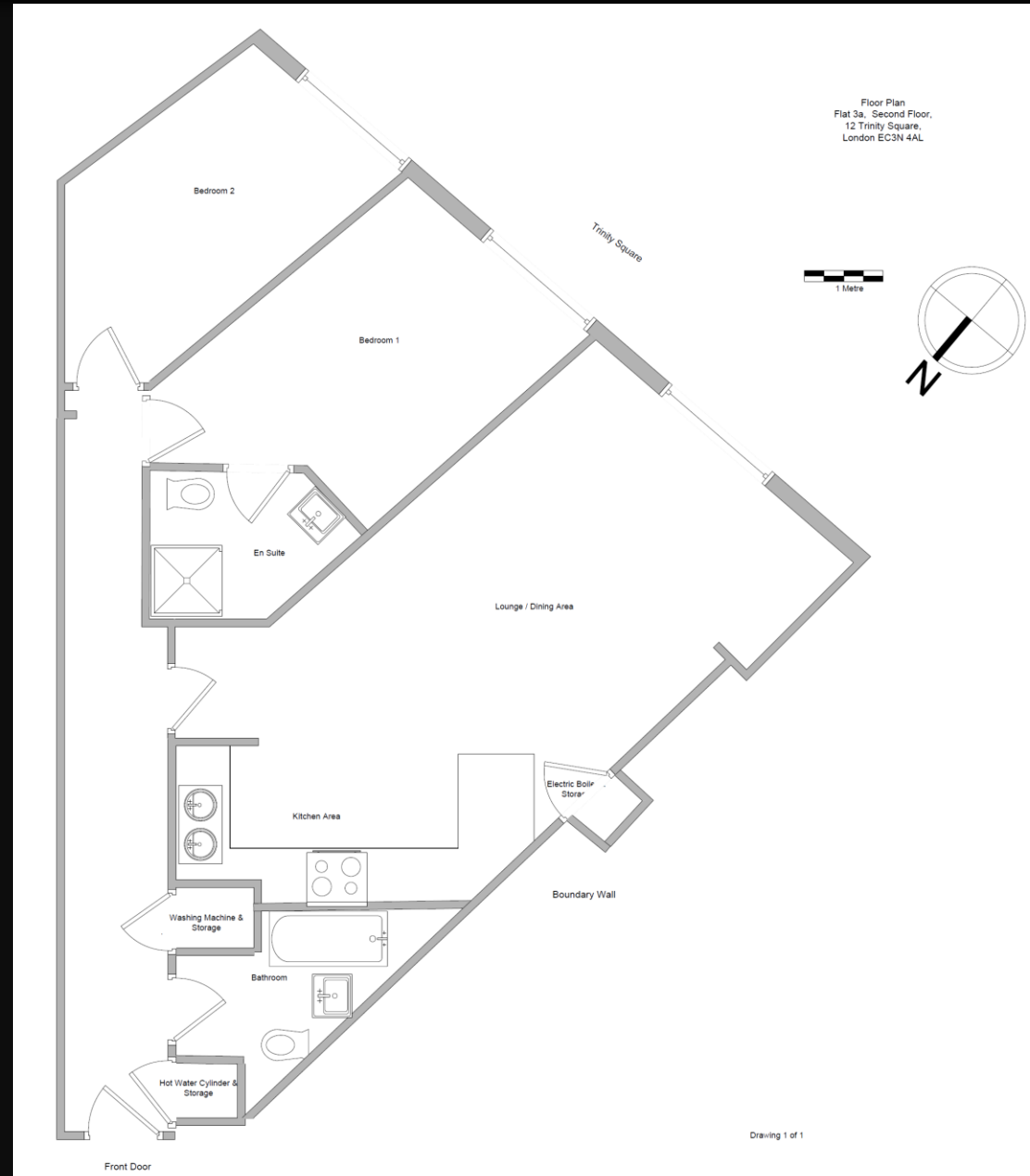
Current Flat Layout Plan
