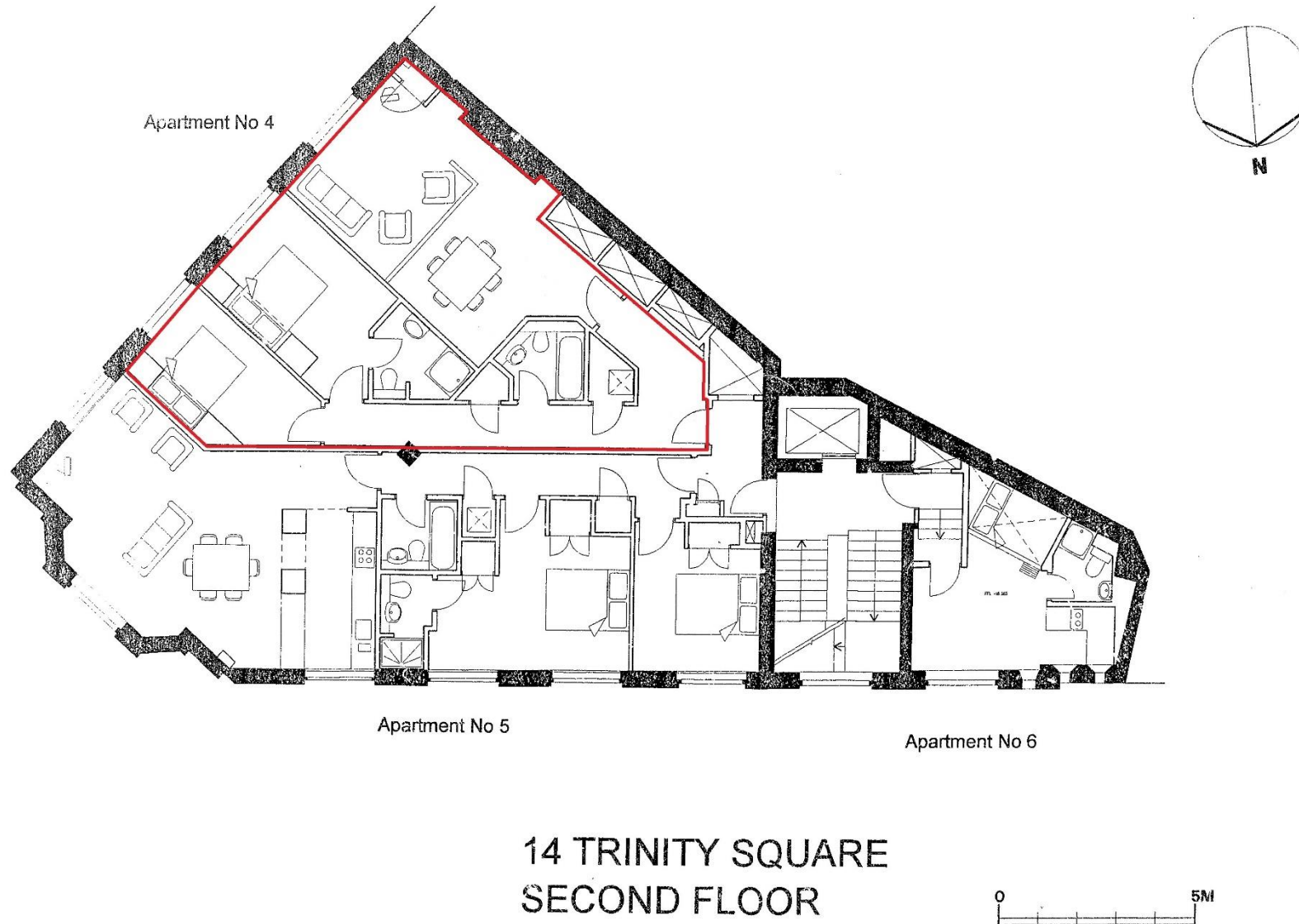
Second Floor Plan (as approved in 1998)
